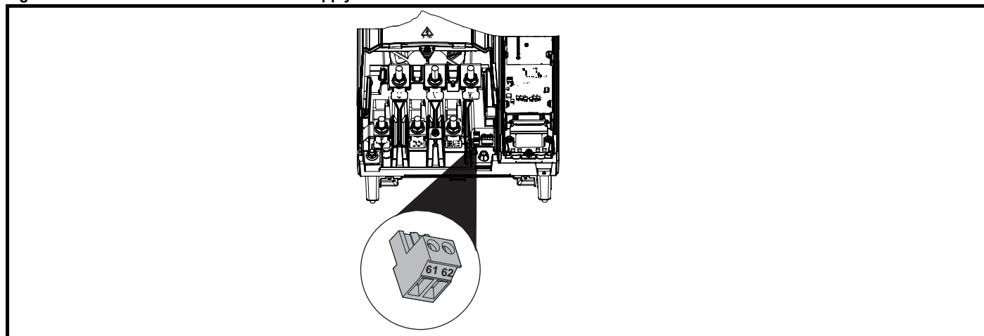
Figure 4-20 Location of the heatsink fan supply connector on size 9 to 11
